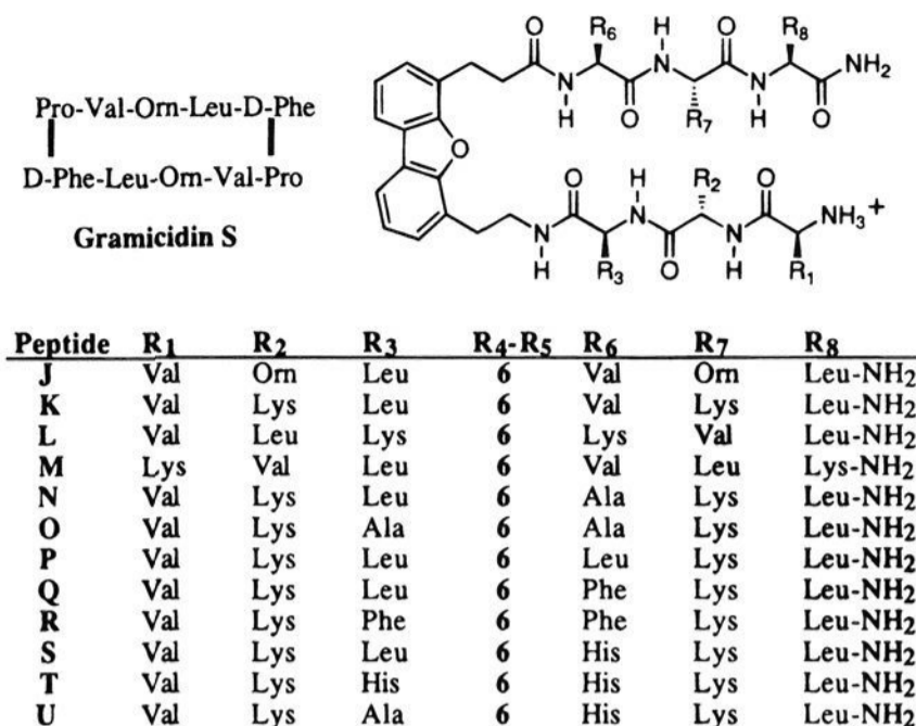
Figure 19. Heptapeptides J–U incorporating the 4-(2-aminoethyl)-6-dibenzofuranpropionic acid residue ( 6 ) are conceptually based on the antibiotic gramicidin S where one of the turn regions (D-Phe-Pro) is excised and the other is replaced with template 6 ; R = \alpha -amino acid side chain.
