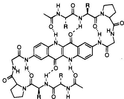
Figure 16. The attachment of peptide strands to the epindolidione amino groups affords a parallel \beta -sheet mimic. Sequences such as Pro-D-Ala are often incorporated proximal to the epindolidione skeleton in order to enforce a reverse turn conformation on the attached peptide which is critical for \beta -sheet formation.
