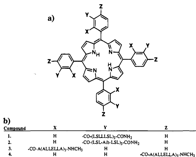
Figure 2. (a) Structure of the tetraphenylporphyrin template used to direct the folding of attached peptide strands into a four-helix bundle and (b) sequence of peptides appended to the ortho, meta, and para positions of the four phenyl functionalities affording tetraphilins 1–4.
