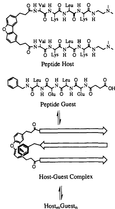
Figure 22. Structure of the host molecule containing a 2,8-dibenzofurandiylbis(3-propanoic acid) residue and the guest peptide. The specificity of the binding event results from favorable hydrophobic interactions as well as electrostatic interactions resulting from the formation of the host-guest complex. After the initial binding event takes place, the complex further self-associates to form soluble \beta -sheet quaternary structure.
