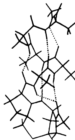
Figure 14. A line drawing of a template-nucleated helix. The template is the (te) conformation and the nucleated helix adopts a structure described by the authors as a 3_{10} - \alpha -helix hybrid where first two residues adjacent to template 5 forms a bifurcated hydrogen bond with the acetamide carbonyl.
